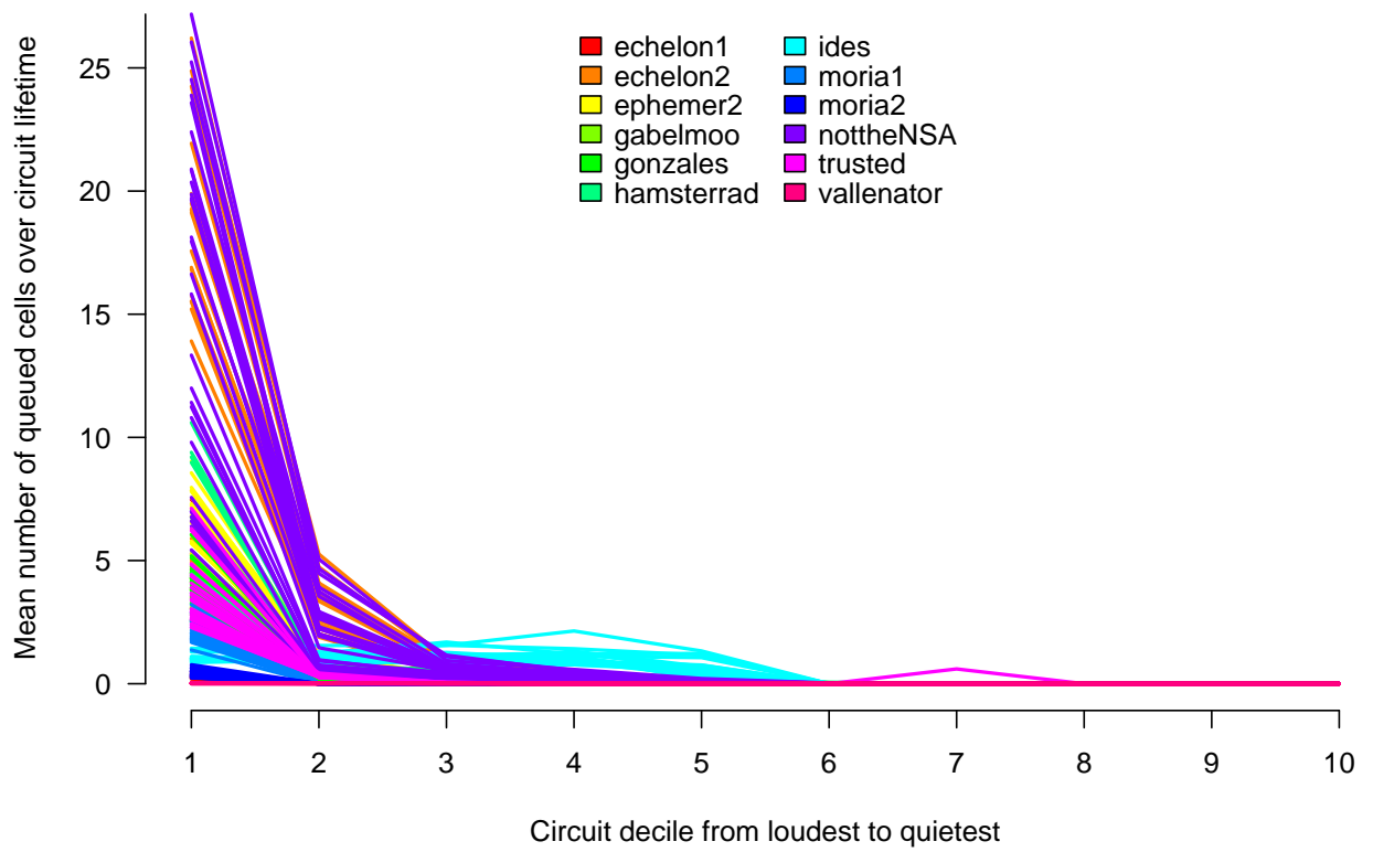
Figure 3: Mean number of cells in queues
